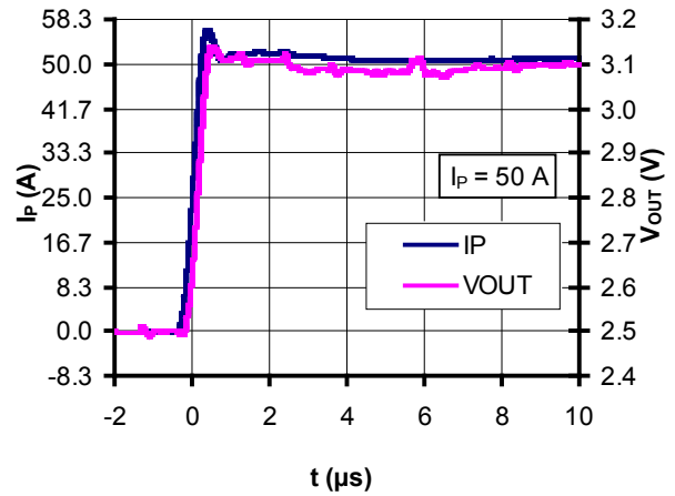
Figure 22: Step response
